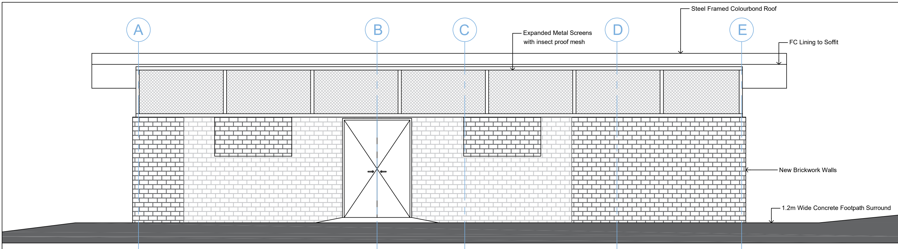
03 001 East Elevation 1:50
