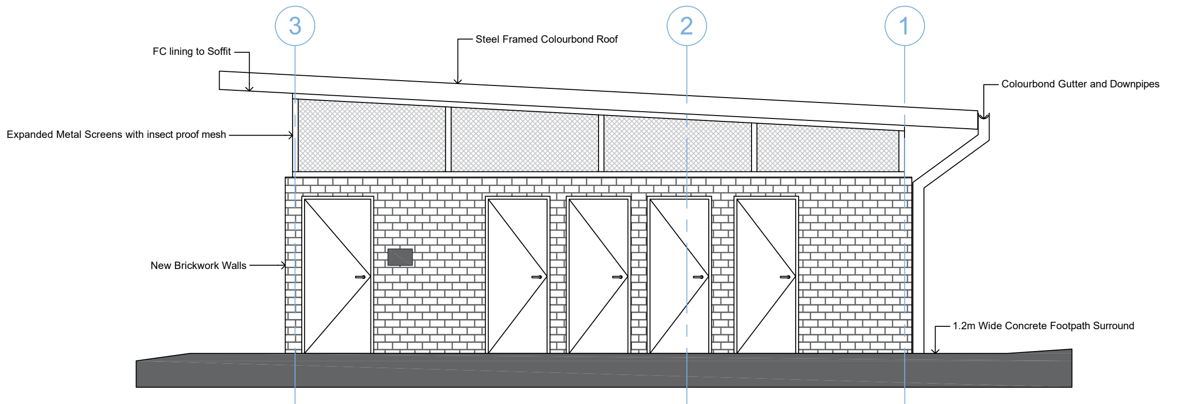
03 002 North Elevation 1:50
