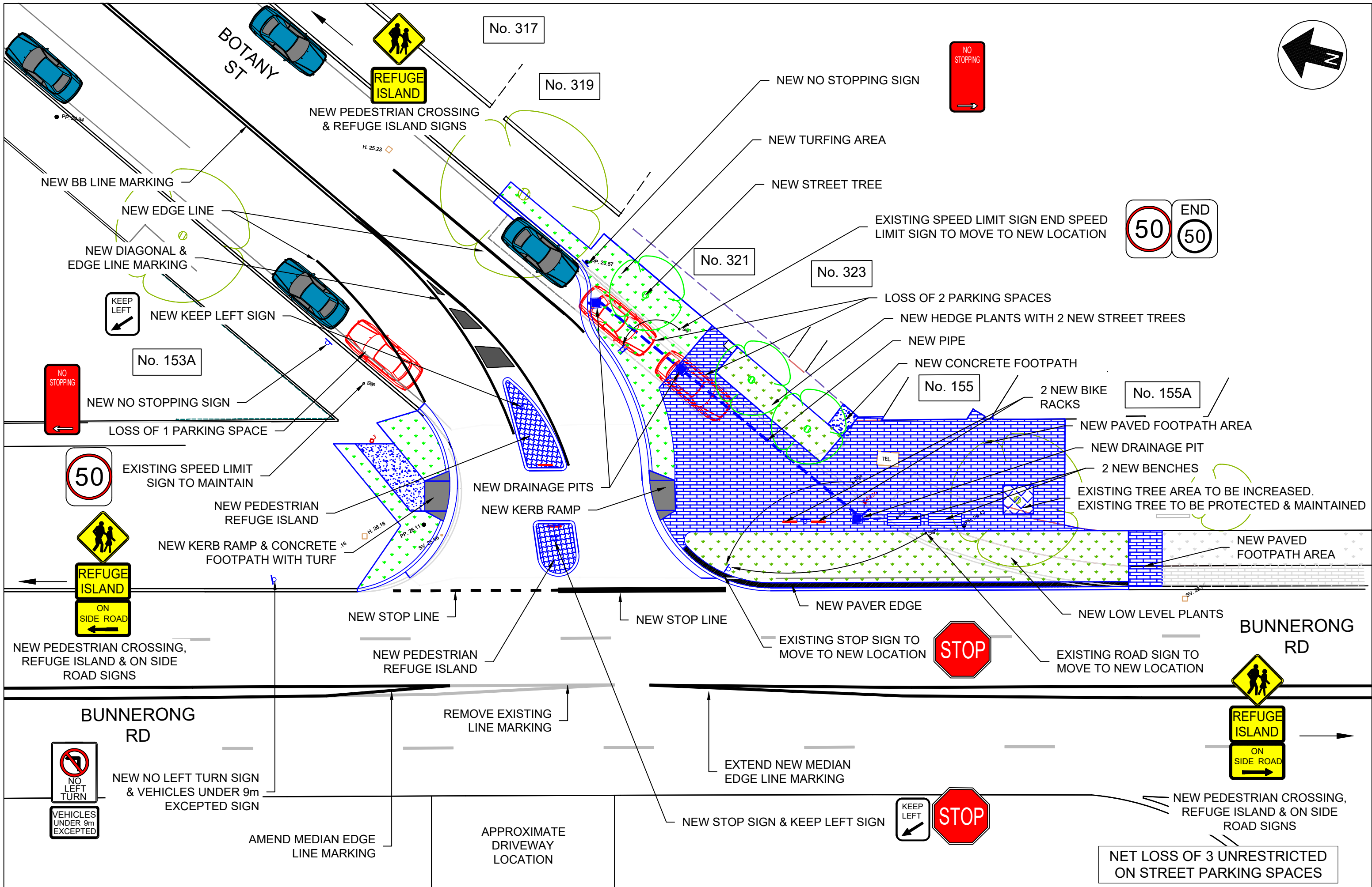
PROPOSED PEDESTRIAN REFUGE INTERSECTION OF BUNNERONG RD AND BOTANY ST, PAGEWOOD NOT TO SCALE
