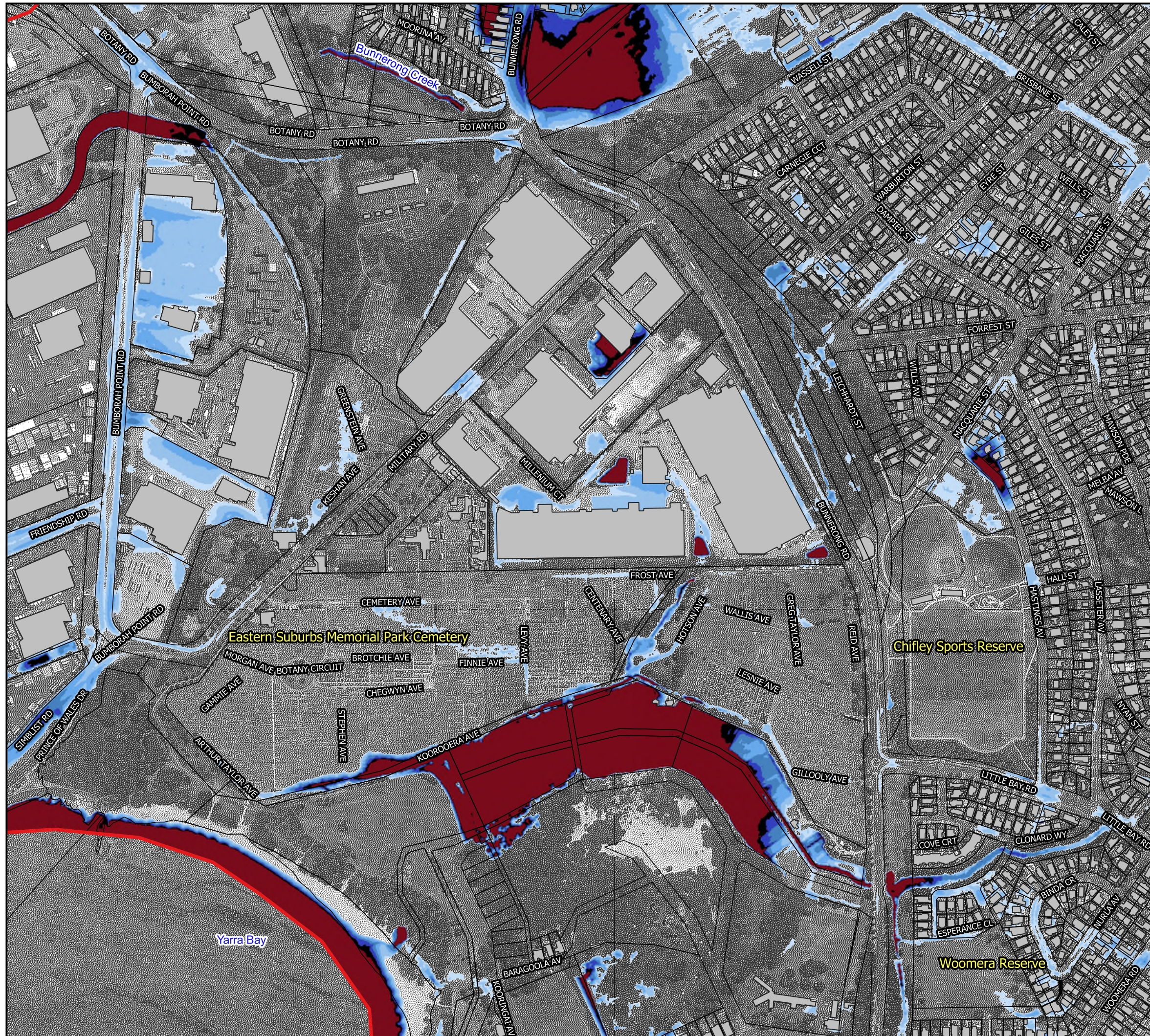
Figure 21.4: Peak Water Depths for the 1% AEP Flood
