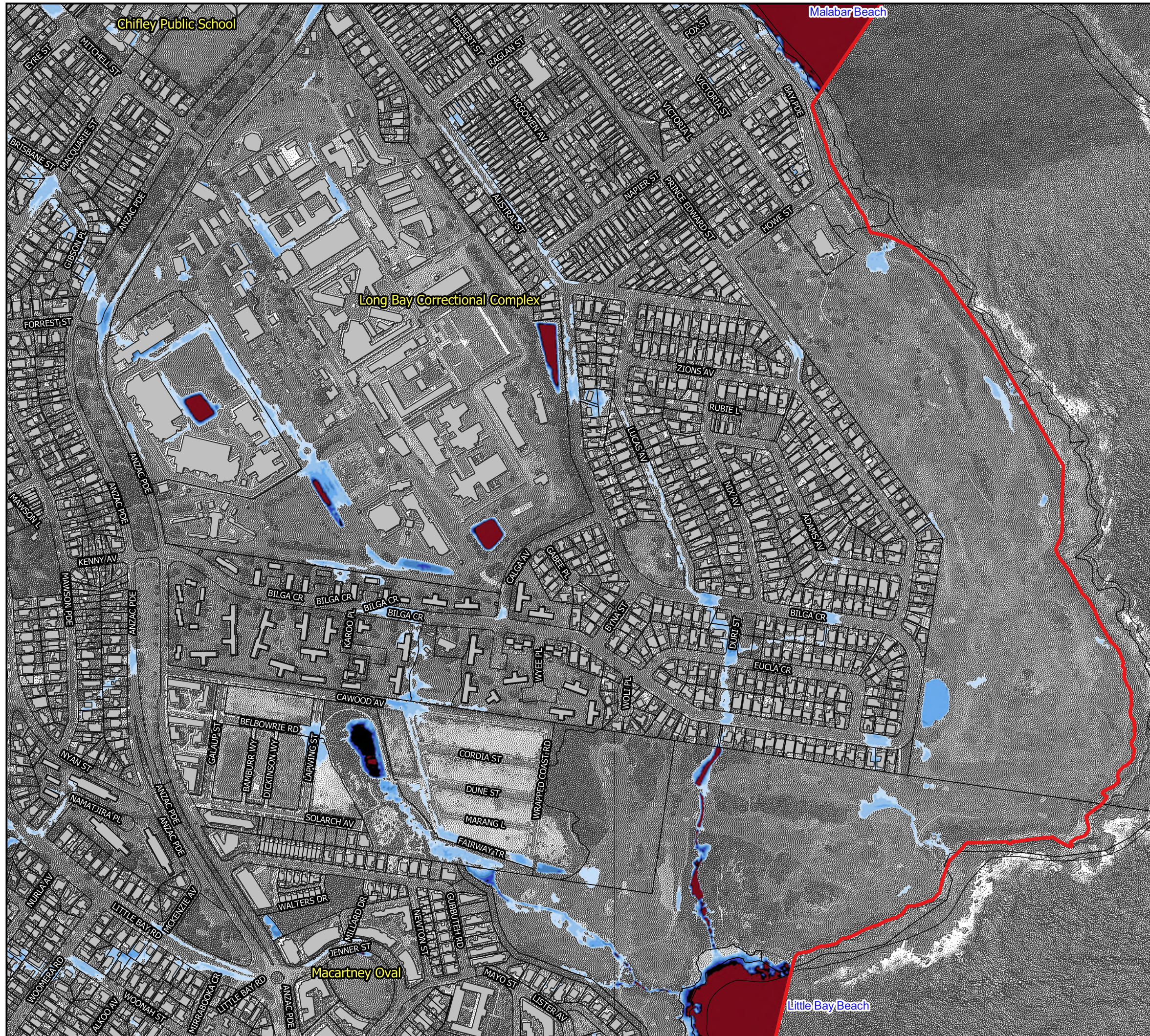
Figure 20.5: Peak Water Depths for the 2% AEP Flood
