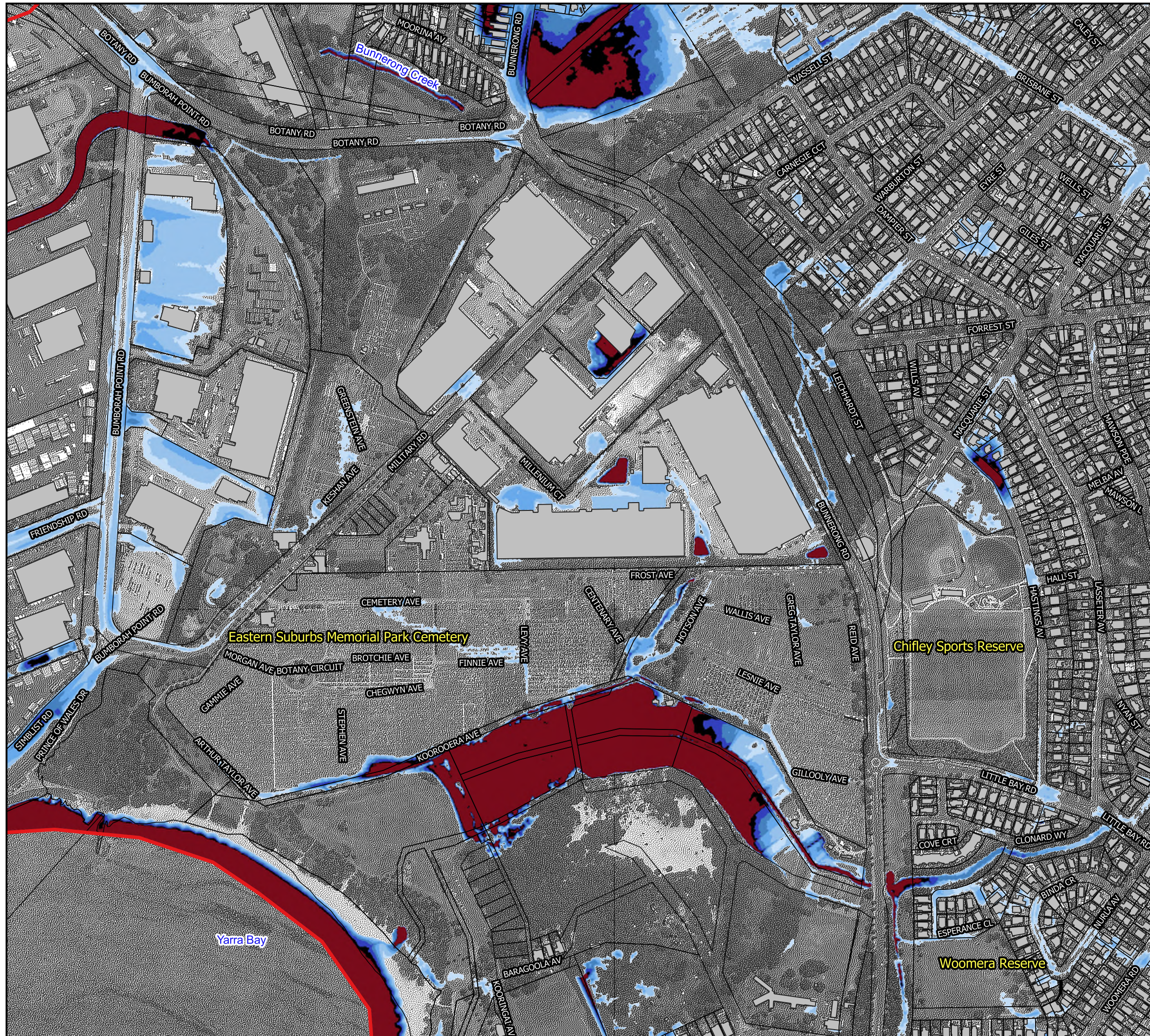
Figure 20.4: Peak Water Depths for the 2% AEP Flood
