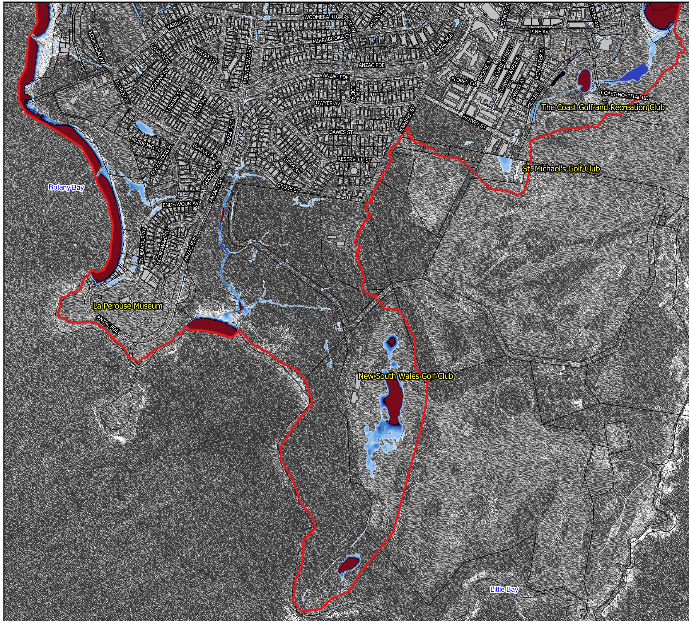
Figure 21.6: Peak Water Depths for the 1% AEP Flood
